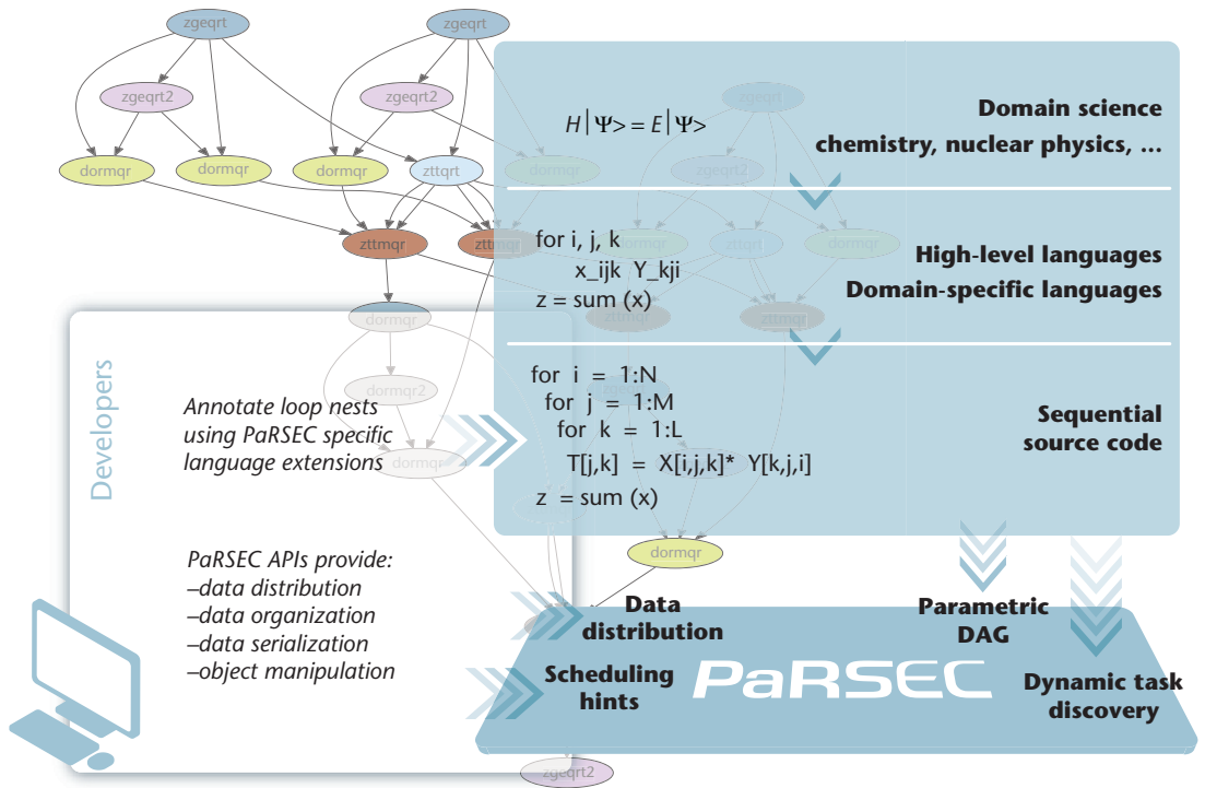
Figure 4. The PaRSEC environment. At a high level, productivity tools convert domain-specific codes into a dataflow representation. The dataflow representation is combined with the PaRSEC runtime library to form the versatile application representation.
